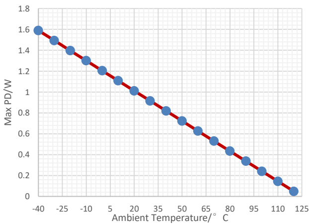
Figure 28. Maximum Allowed Power Dissipation vs Ambient Temperature, SOT23-5, T_J \leq 125^\circ\text{C}
