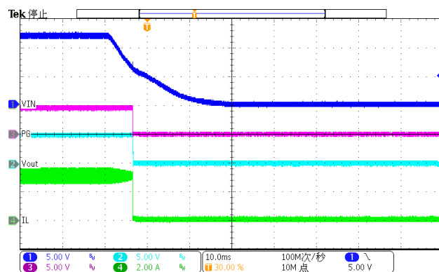
Figure 14. Power down (Iload=3A)
