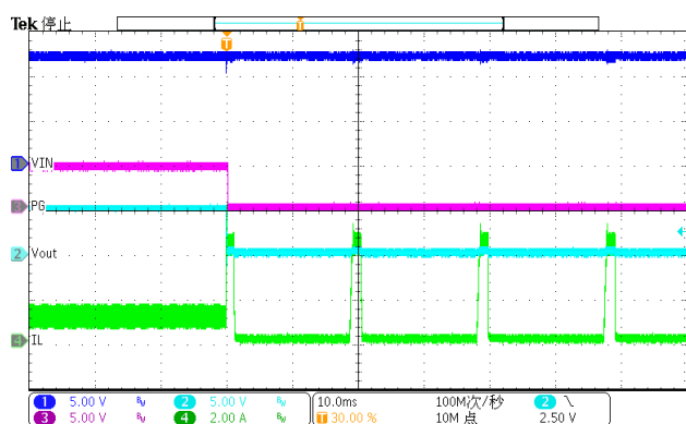
Figure 17. Normal to Hard Short
