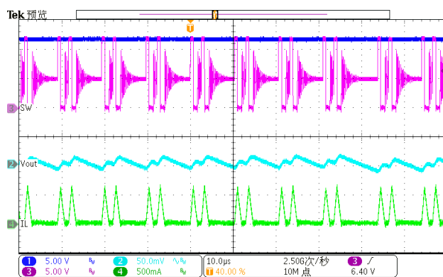
Figure 22. Output Ripple (Iload=0.1A)
