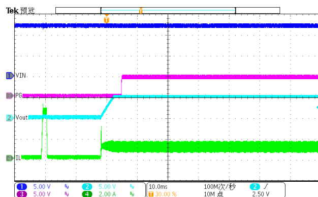
Figure 18. Hard Short Recovery
