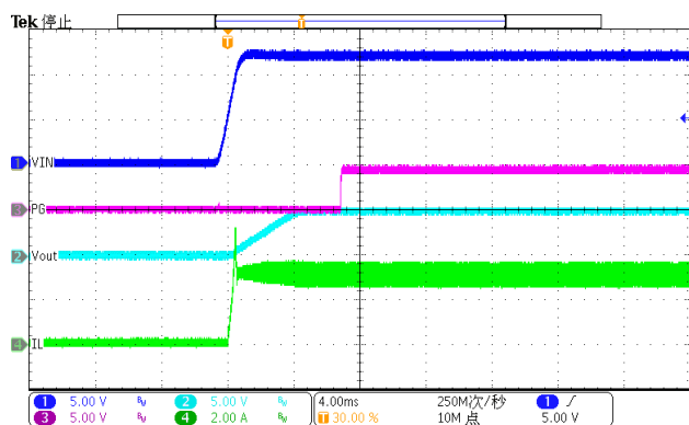
Figure 13. Power up (Iload=3A)
