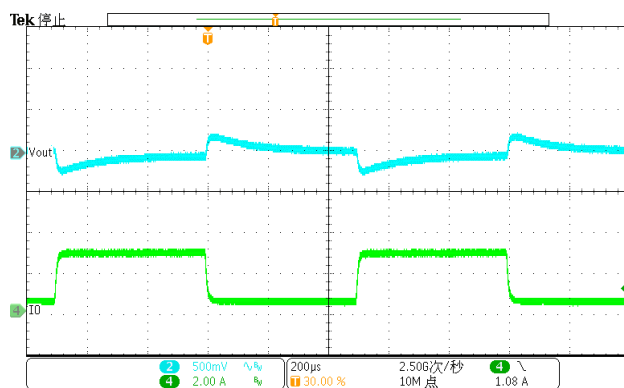
Figure 20. Load Transient (0.3A-2.7A, 1.6A/us)
