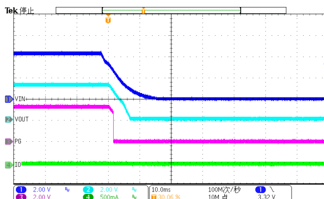
Figure 34. Power down (Iload=10mA)
