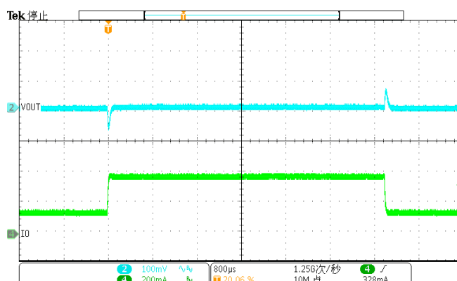
Figure 38. DC-DC Load Transient (130mA-370mA), VOUT=3.3V
