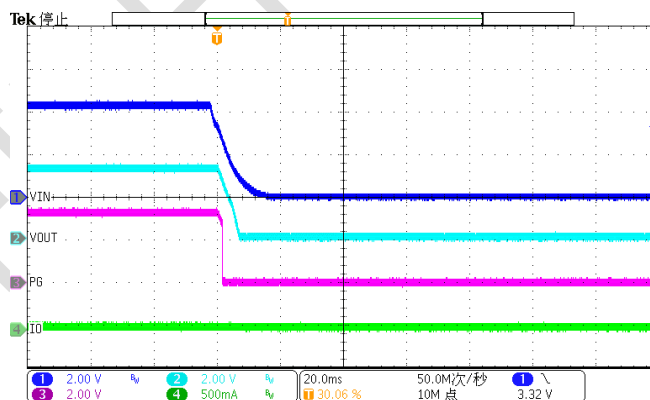
Figure 36. Slow Power down (Iload=10mA)
