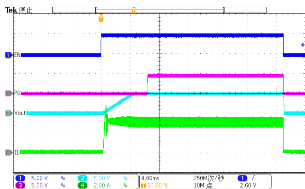
Figure 15. Enable (Iload=3A)
