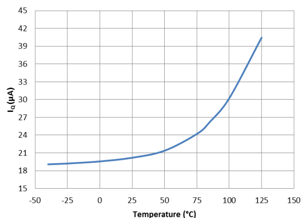
Figure 6. IQ vs. Temperature, IOU = 0A
