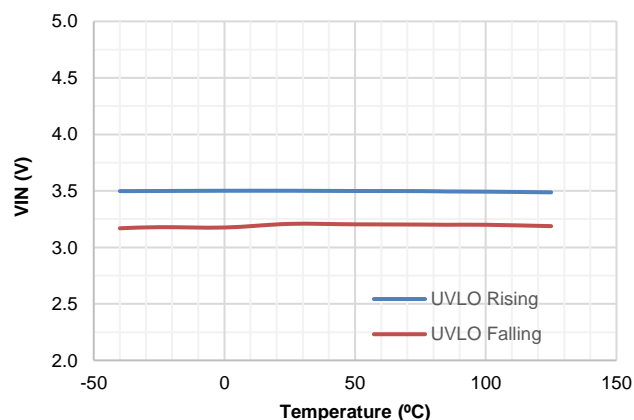
Figure 4. VIN UVLO vs Temperature
