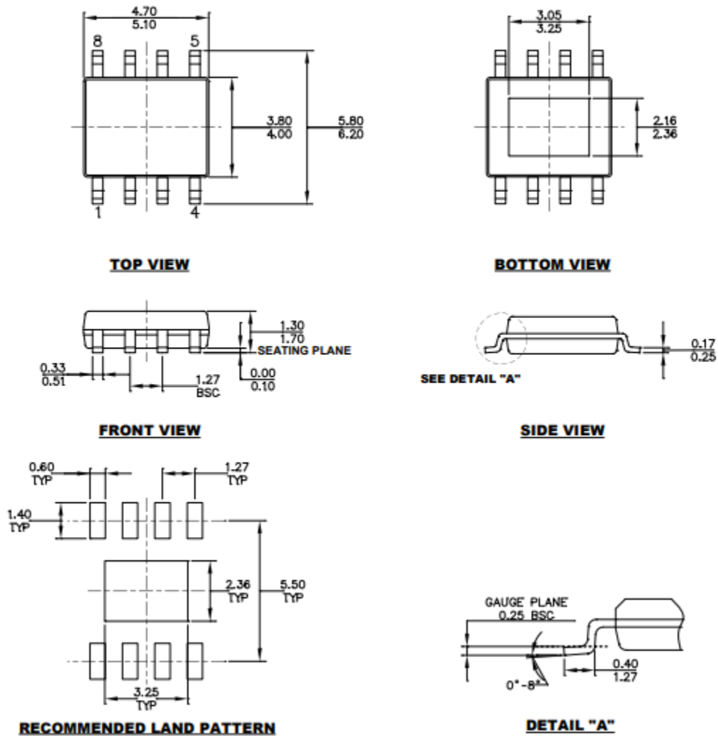
ESOP-8 Package Outline Dimensions
