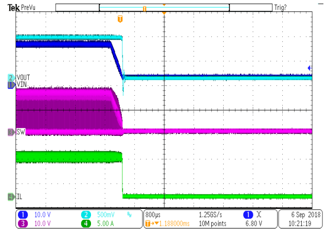
Figure 9. Power Down
