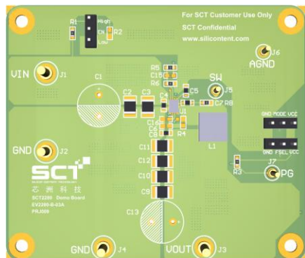
EV2280-B-04A Evaluation Board Top View
