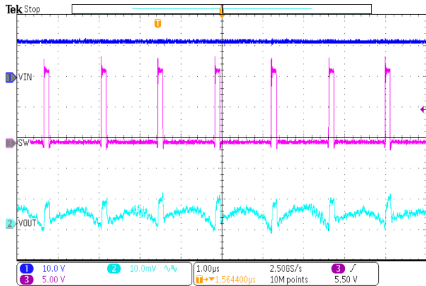
Figure 10. Steady State Ripple Iout=2A
