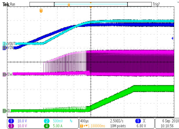
Figure 8. Power Up
