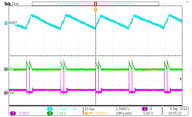
Figure 11. Steady State Ripple Iout=600mA
