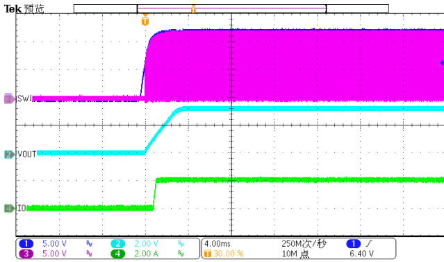
Figure 9. Power up(Iload=2A)
