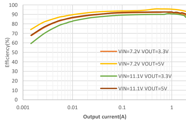
SCT2230M Efficiency
