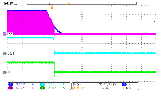
Figure 10. Power down(Iload=2A)
