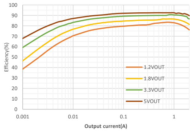
Figure 2. Efficiency vs Load Current(VIN=11.1V)
