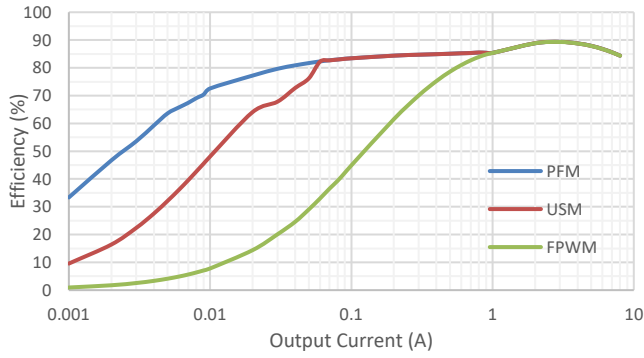
Figure 2. Efficiency V_{IN}=12V, V_{out}=1V, F_{sw}=400kHz SCT22C1C
