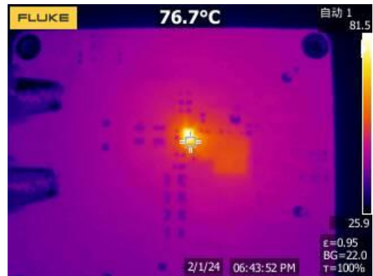
Figure 34. Thermal, 12 VIN, 1 Vout, 8A
