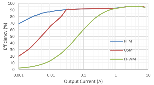
Figure 7. Efficiency V_{IN}=12V, V_{out}=1V, F_{sw}=1200kHz SCT22C0C
