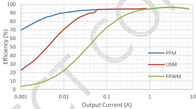
Figure 6. Efficiency V_{IN}=12V, V_{out}=1V, F_{sw}=800kHz SCT22C0C
