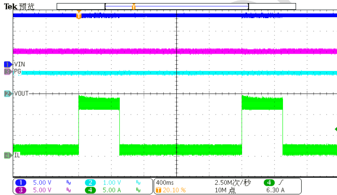
Figure 33. Output Ripple (Iload=8A)
