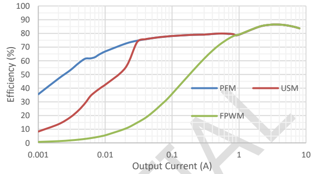
Figure 3. Efficiency V_{IN}=12V, V_{out}=1V, F_{sw}=800kHz SCT22C1C
