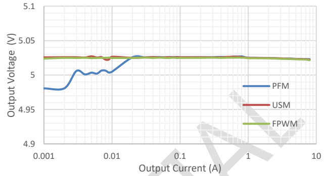
Figure 9. Load Regulation, Vout=5V Fsw=400kHz SCT22C0C
