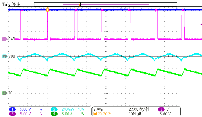
Figure 31. Output Ripple (Iload=8A) 400kHz
