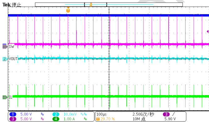
Figure 27. Output Ripple (Iload=10mA, USM)
