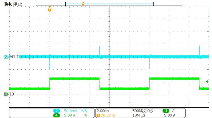
Figure 30. Load Transient (2A-6A, 1.6A/us)
