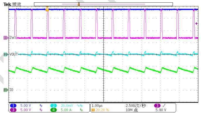
Figure 32. Output Ripple (Iload=8A) 1200kHz
