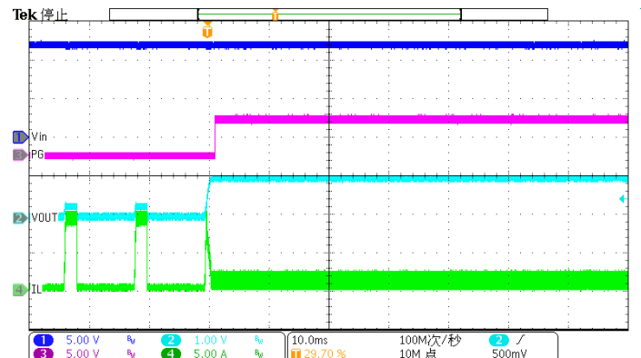
Figure 22. Over Current Release (hard short to 1A)
