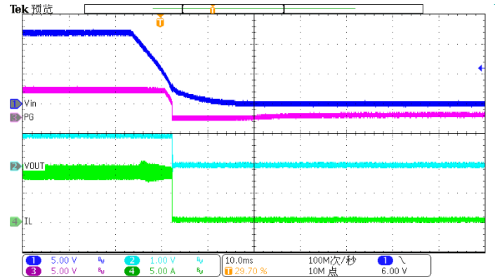
Figure 18. Power down
