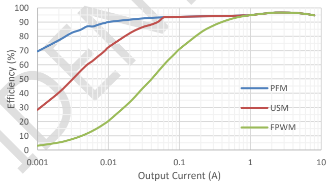
Figure 5. Efficiency V_{IN}=12V, V_{out}=5V, F_{sw}=400kHz SCT22C0C
