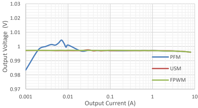
Figure 8. Load Regulation, Vout=1V Fsw=400kHz SCT22C1C
