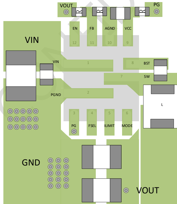
Figure 35. PCB Layout Example
