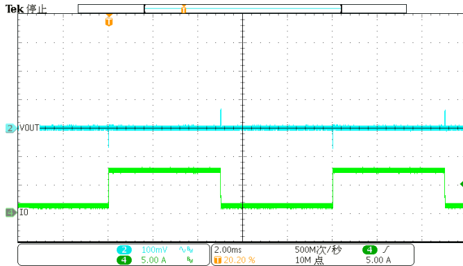
Figure 29. Load Transient (0.8A-7.2A, 1.6A/us)
