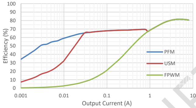
Figure 4. Efficiency V_{IN}=12V, V_{out}=1V, F_{sw}=1200kHz SCT22C1C
