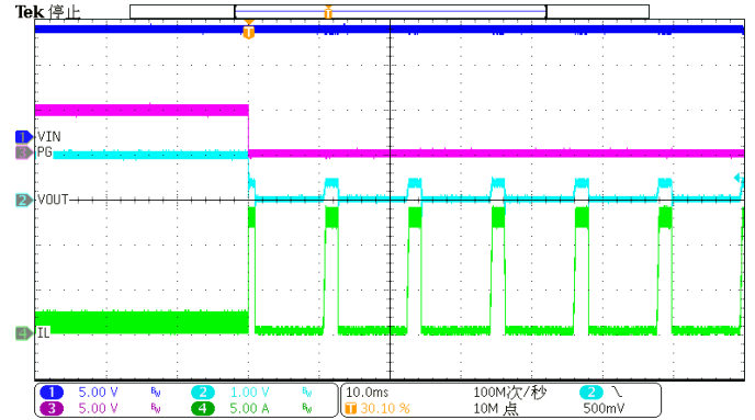
Figure 24. Over Current Protection ILIMIT=14A
