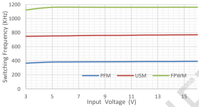
Figure 10. Switching Frequency VS Input Voltage
