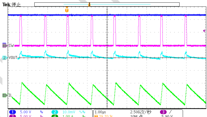
Figure 26. Output Ripple (Iload=10mA, FPWM)
