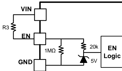
Figure 7. Adjustable VIN UVLO
