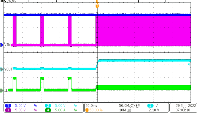
Figure 14. Over Current Release (1A to hard short)
