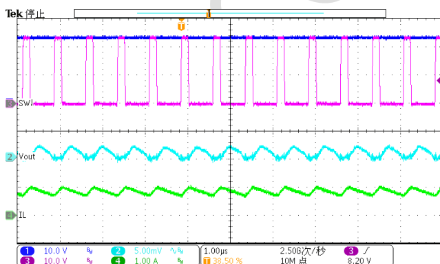
Figure 28. Output Ripple (ILOAD=0.8A)
