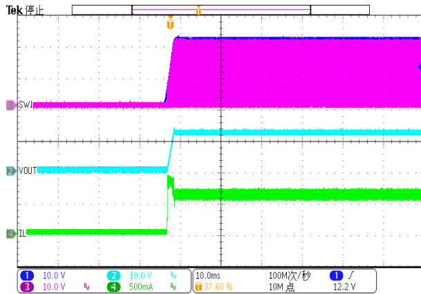
Figure 19. Power up
