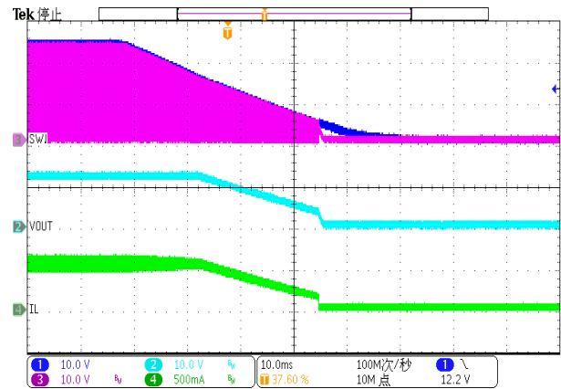
Figure 20. Power down
